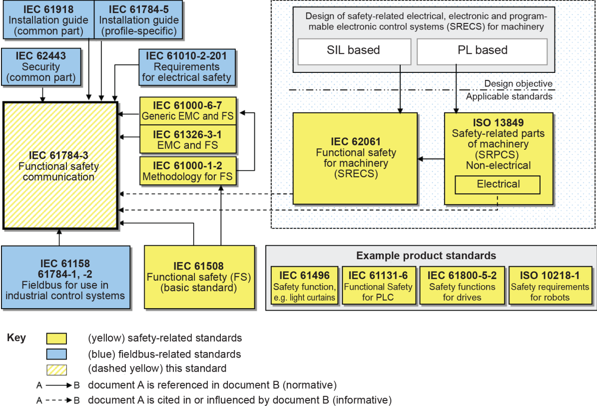
Figure 1 shows the relationships between IEC 61784-3 (all parts) and relevant safety and fieldbus standards in a machinery environment.
